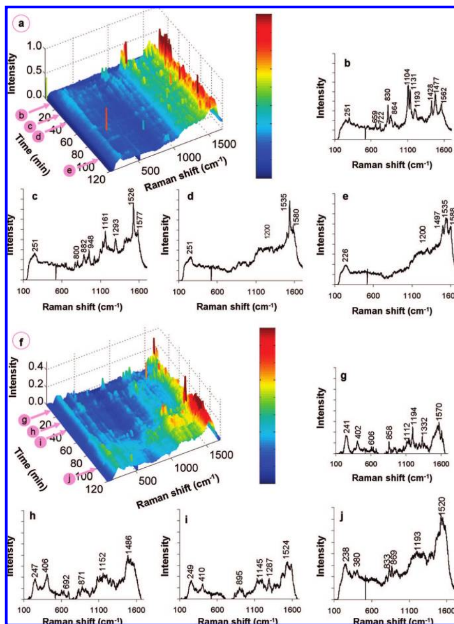
Figure 4. (a) Waterfall plot of time-resolved spectra gathered from the reaction of 50.9 \mu\text{M} 1,1-DCE and 16.3 \text{ mM H}_2 on Pd/Au NSs, and individual scans at 12, 30, 41, and 100 min (b, c, d, and e, respectively) after injection of 1,1-DCE/ \text{H}_2 solution. (f) Waterfall plot of time-resolved spectra gathered from the reaction of 254 \mu\text{M} 1,1-DCE and 81.9 \text{ mM H}_2 on Pd/Au NSs, and individual scans at 12, 30, 41, and 100 min (g, h, i, and j, respectively) after injection of 1,1-DCE/ \text{H}_2 solution.
