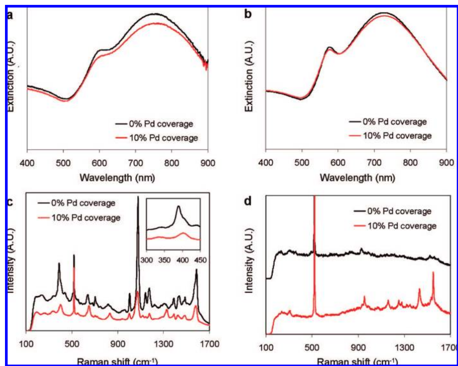
Figure 2. (a) UV-vis spectra of Au NS and Pd/Au NS (10% Pd coverage); (b) calculated spectra of Au and Pd/Au NS; (c) spectra of pMA chemisorbed on Au NS and Pd/Au NS (10% Pd coverage) (inset: metal-S stretching region); (d) 1,1-DCE in H 2 O (50.9 μM) on Au NS and Pd/Au NS (10% Pd coverage) (spectra offset for clarity). The Raman peak at ~500 cm -1 comes from the Si wafer, and small peaks in the 900–1000 and 1400–1600 cm -1 regions are from organic residuals prior to contact with 1,1-DCE.
