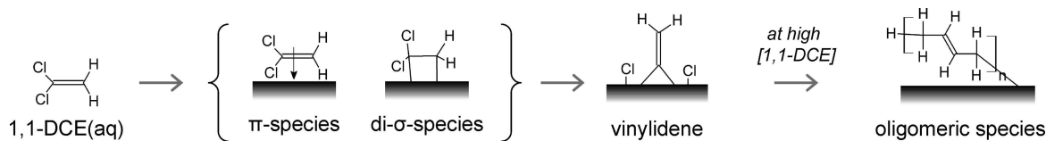
Scheme 1. Proposed Surface Intermediates of 1,1-DCE after Adsorption on Pd/Au NS SERS Substrate Based on Spectroscopic Results a
