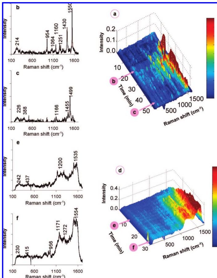
Figure 3. (a) Waterfall plot of time-resolved spectra gathered from the chemisorption of 50.9 \mu\text{M} 1,1-DCE on Pd/Au NSs and (b,c) individual scans at 20 and 49 min after injection of 1,1-DCE solution. (d) Waterfall plot of time-resolved spectra gathered from the chemisorption of 254 \mu\text{M} 1,1-DCE and (e,f) individual scans at 10 and 28 min after injection of 1,1-DCE solution.
