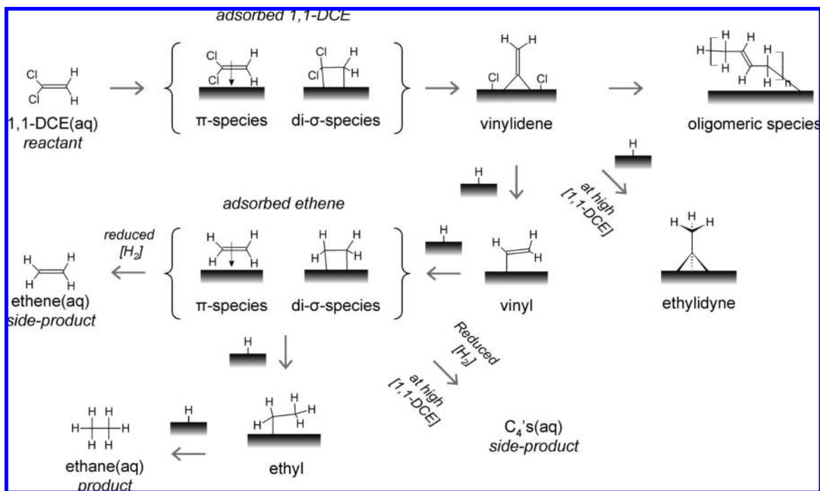
Scheme 2. Proposed Surface Intermediates of 1,1-DCE and H 2 under Reactive Conditions on Pd/Au NS SERS Substrate Based on Spectroscopic Results a
